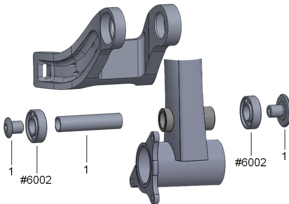
1 - Kit 2: Main Pivot Link
