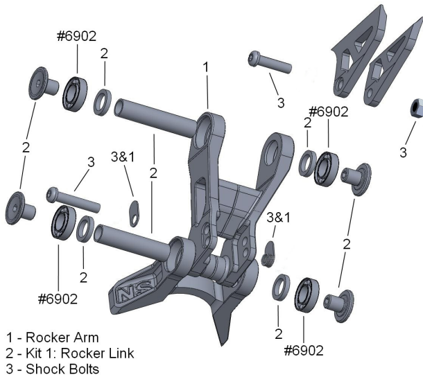
Fig. 2 Soda frame rocker arm links details
